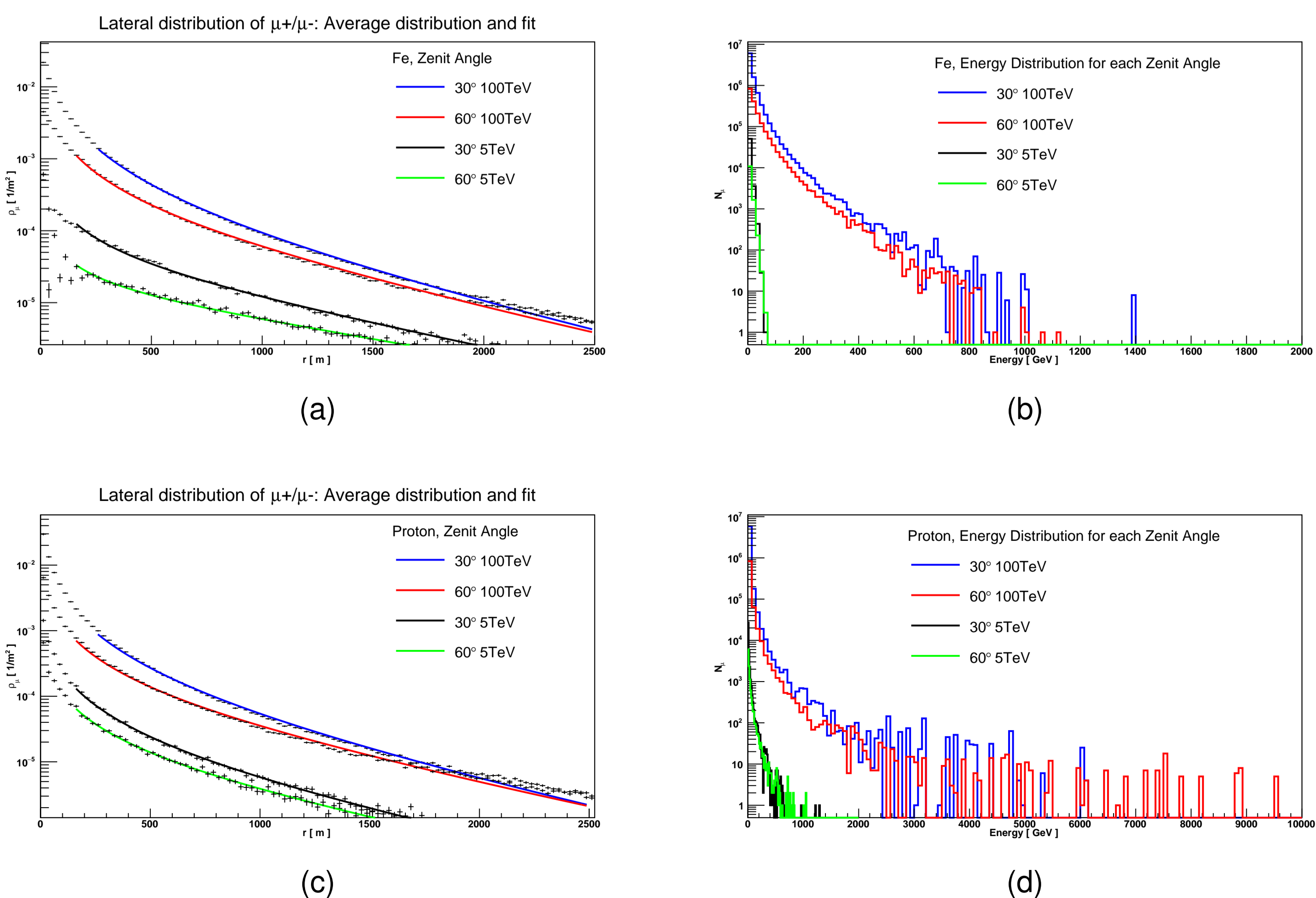
Number of muons per m^2 from a Fe Nucleus (a) and protons (c).
