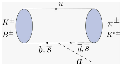
Figure 1: Tree level diagram contribution to the FCNC processes K^\pm \rightarrow \pi^\pm a and B^\pm \rightarrow K^{*\pm} a .
