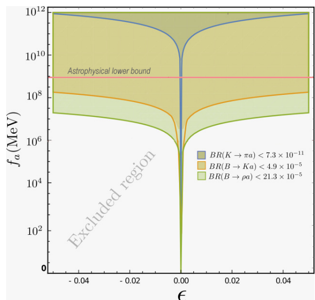
Figure 2: Allowed regions for semileptonic meson decays. We use the relation (1) between the axion mass and the decay constant f_a .
