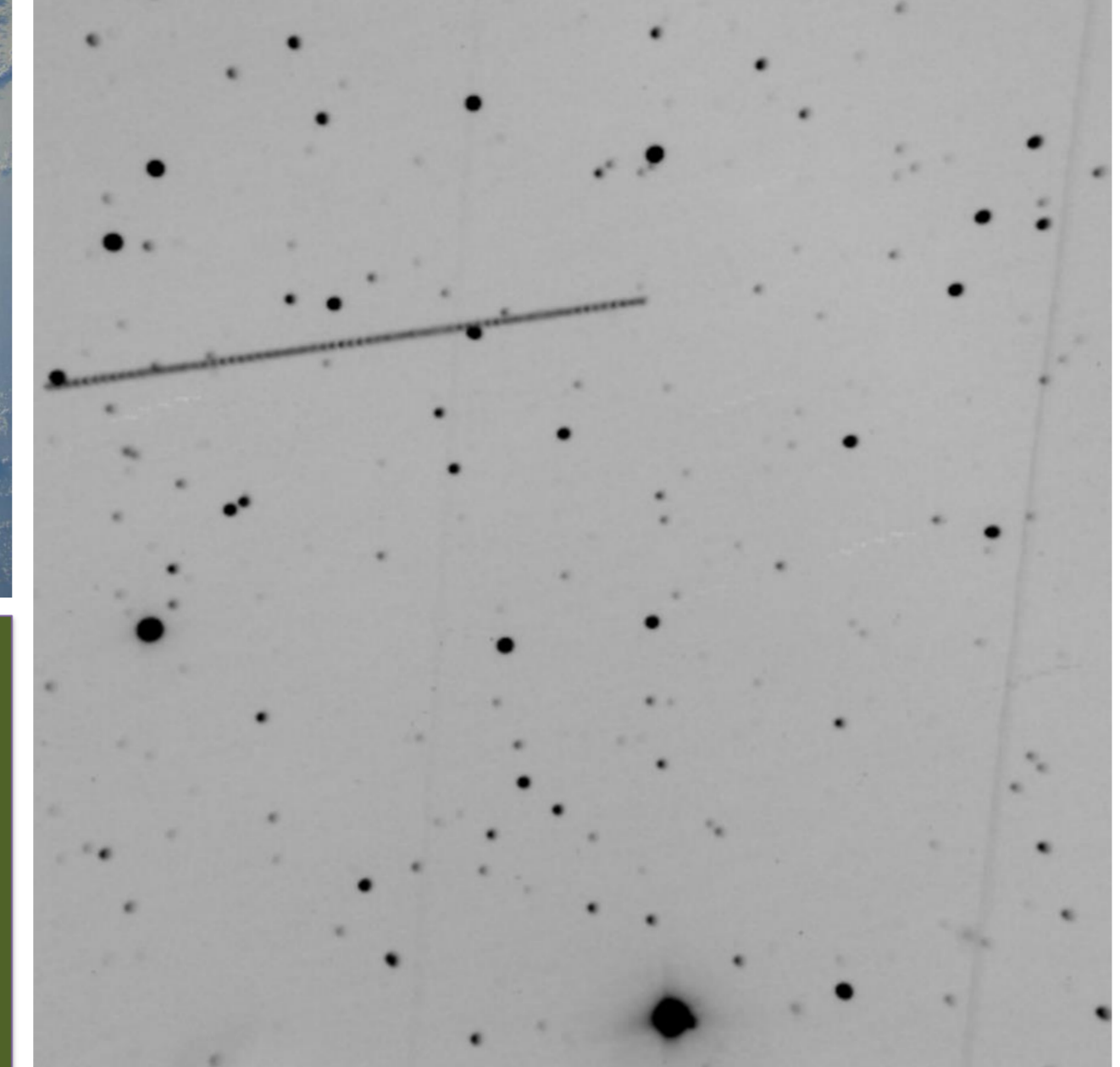
ASTEROID 1998 WT24 December 12 / 2015 By: Alberto Quijano Vodniza & Mario Rojas Pereira University of Narino Observatory - Colombia Interval of time = 26 minutes + 25 seconds Image Scale = 2.35 arcseconds / pixel CGE Pro 1400 CELESTRON telescope & STL-1001E SBIG
